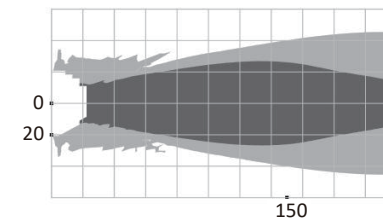
Dark colour: 25mm diameter PVC pipe Light colour: 100mm*100mm flat plate Note: There may be deviation,for reference only
