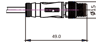
M12 Connector
