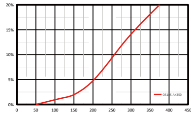
Scanning distance difference Curve (White 90%/black 6%)
