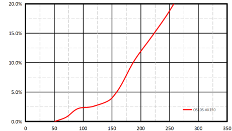
Scanning distance difference Curve (White 90%/black 6%)
