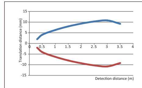
OP18 Polarized retro-reflective
