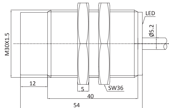
Fig. 1 Inductive sensor with cable (non-flush)
