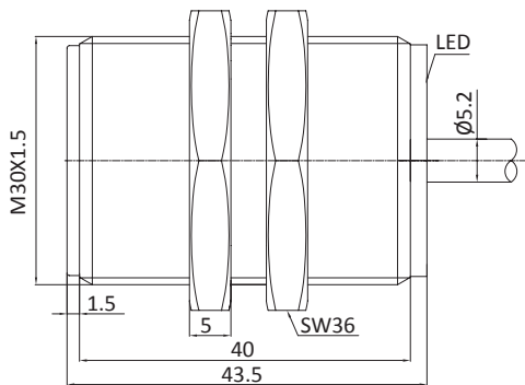
Fig. 1 Inductive sensor with cable (flush)
