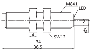
Fig. 1 Inductive sensor with cable (flush)
