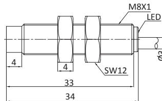
Fig. 1 Inductive sensor with cable (non-flush)
