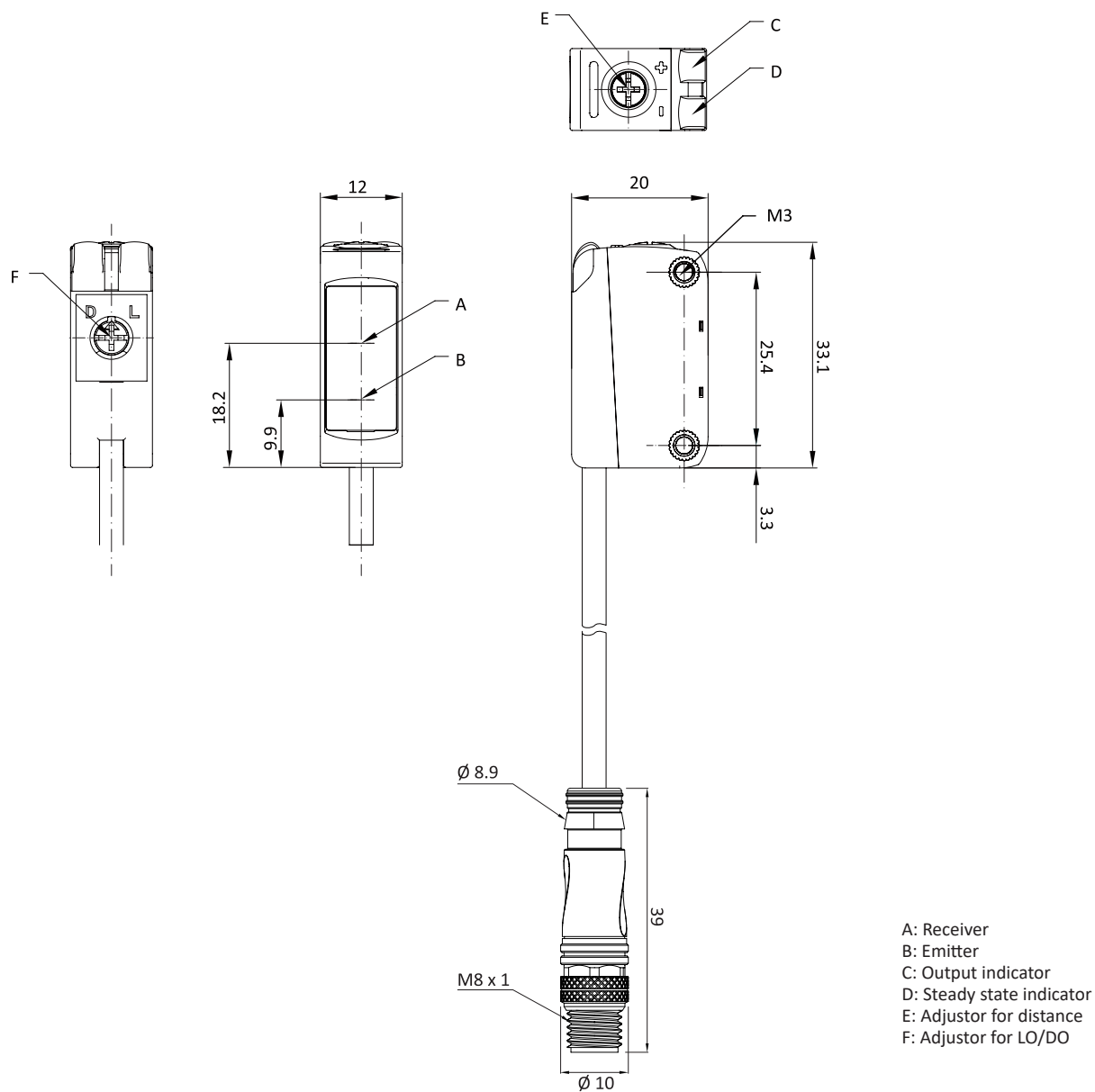
Fig. 3 BGS / diffused
