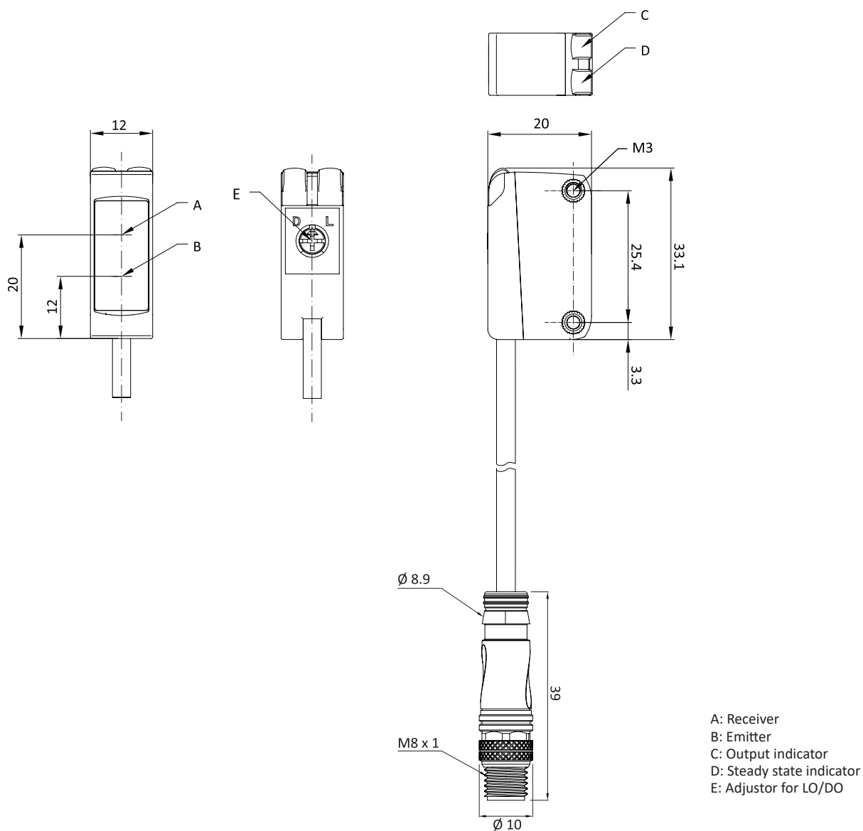
Fig. 2 Polarized retroreflective
