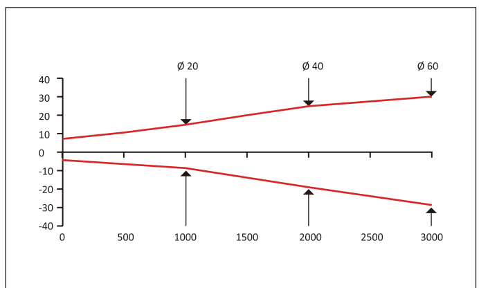
OS10S-PR (mm)
