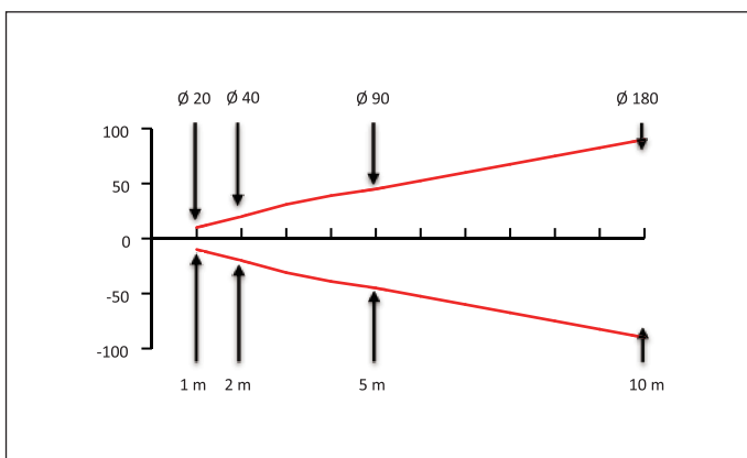
Beam Pattern
