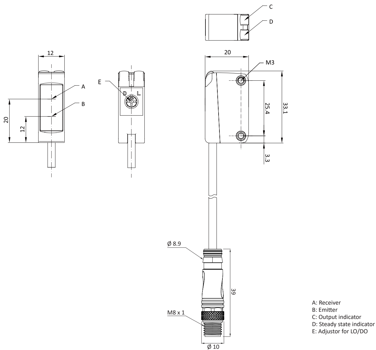
Fig. 2 Polarized retroreflective
