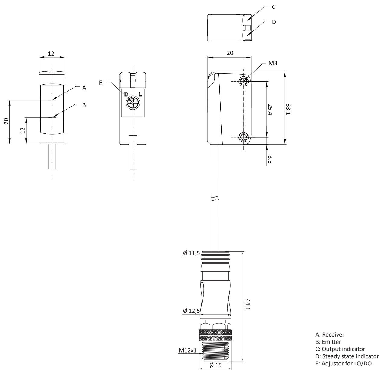
Fig. 2 Polarized retroreflective
