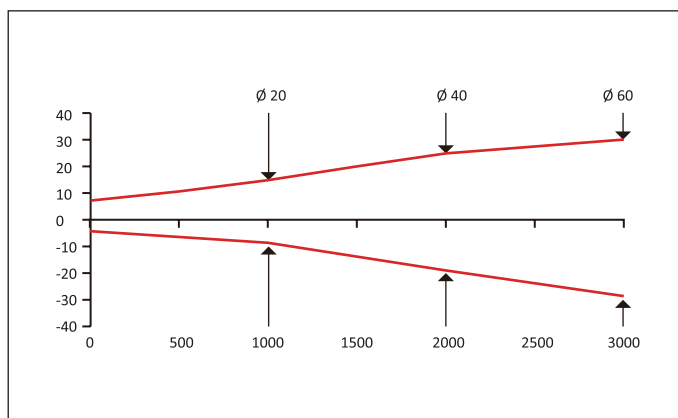
OS10S-PR (mm)
