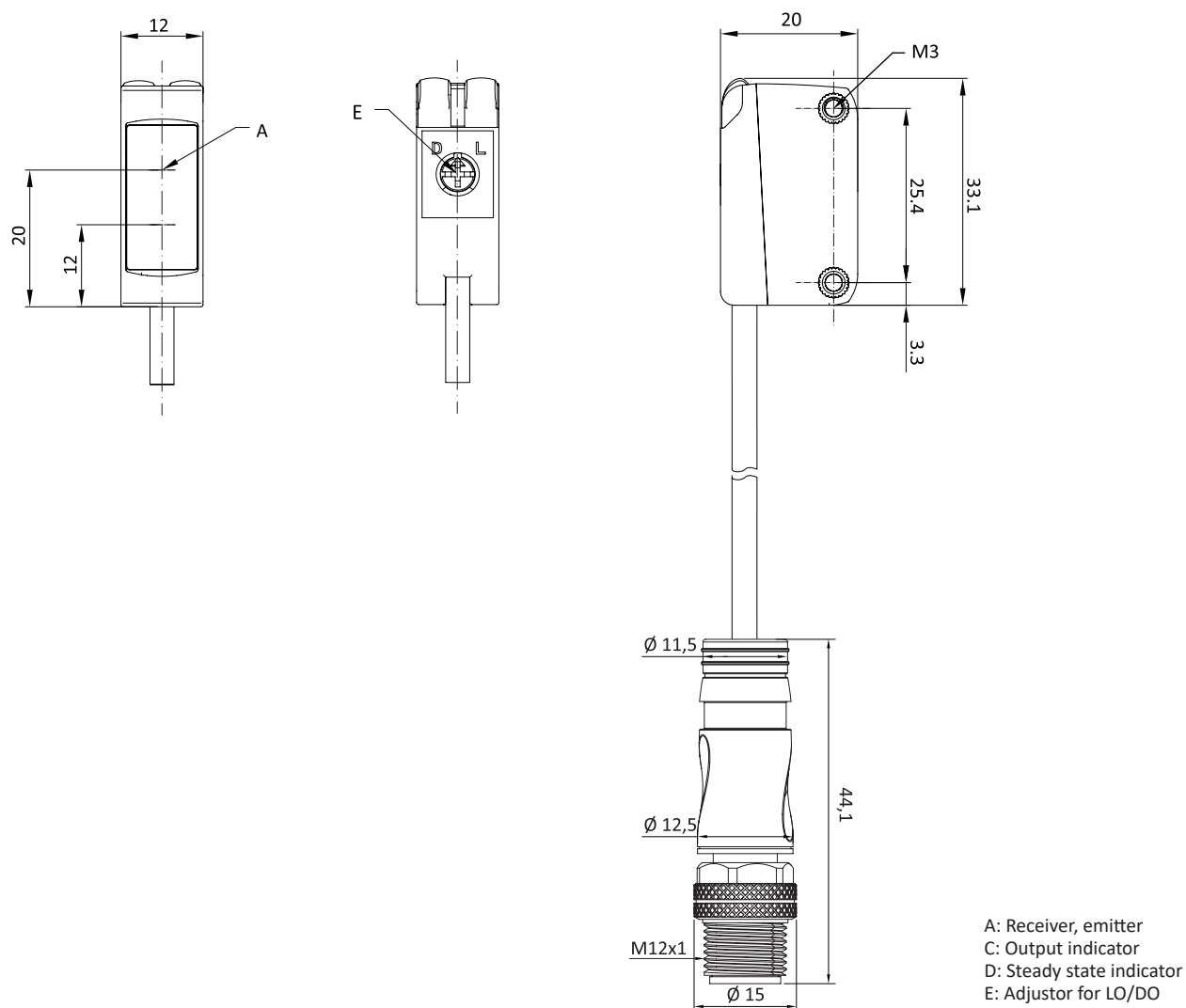
Fig. 1 Opposed
