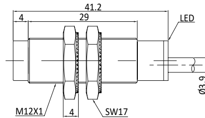
Fig. 2 Inductive sensor with cable (non-flush)
