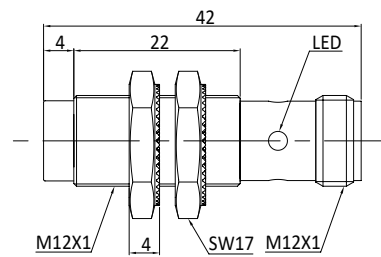
Fig. 4 Inductive sensor with M12 connector (non-flush)
