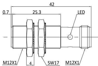
Fig. 3 Inductive sensor with M12 connector (flush)
