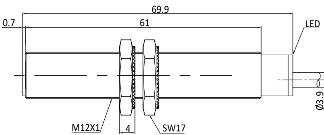
Fig. 5 Inductive sensor with cable (flush)
