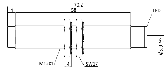
Fig. 6 Inductive sensor with cable (non-flush)
