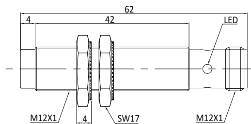
Fig. 8 Inductive sensor with M12 connector (non-flush)
