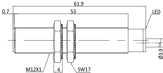
Fig. 3 Inductive sensor with cable (flush)
