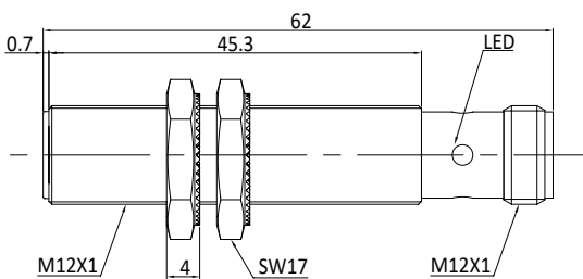
Fig. 7 Inductive sensor with M12 connector (flush)
