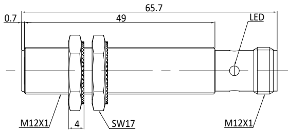
Fig. 9 Inductive sensor with M12 connector (flush)
