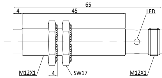
Fig. 10 Inductive sensor with M12 connector (non-flush)
