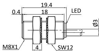
Fig. 1 Inductive sensor with cable (flush)
