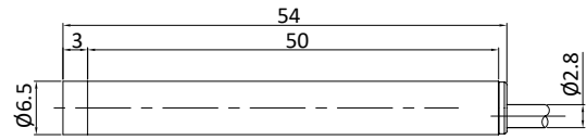
Fig. 2 Inductive sensor with cable (non-flush)
