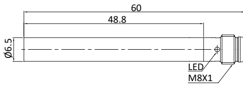
Fig. 3 Inductive sensor with M8 connector (flush)
