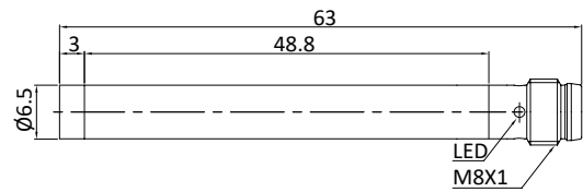
Fig. 4 Inductive sensor with M8 connector (non-flush)
