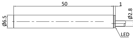
Fig. 1 Inductive sensor with cable (flush)
