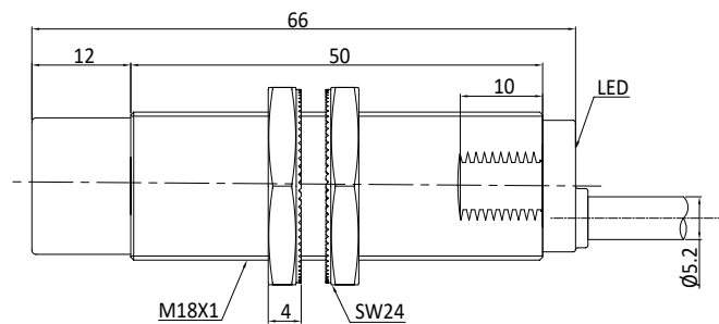
Fig. 1 Inductive sensor with cable (non-flush)
