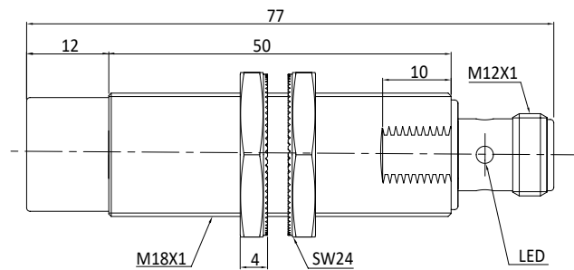
Fig. 2 Inductive sensor with M12 connector (non-flush)
