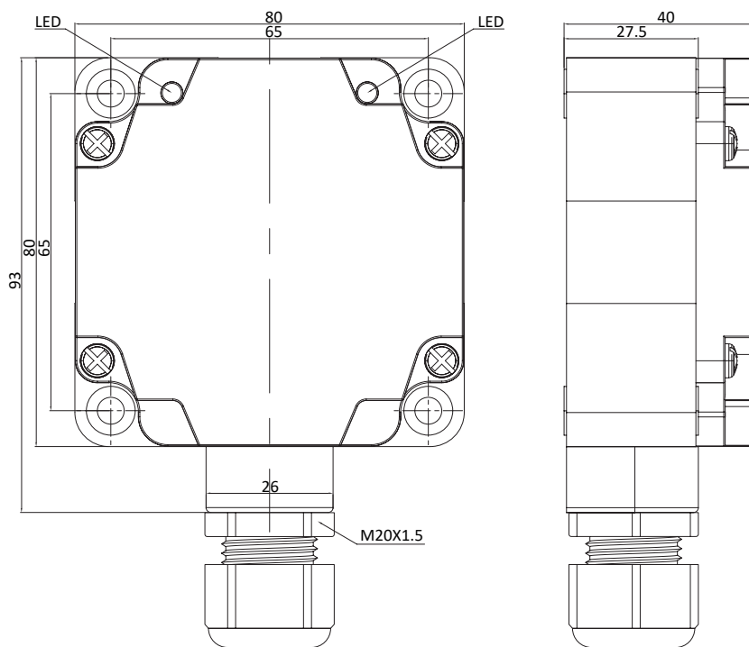
Fig. 1 Inductive sensor with terminals (flush/non-flush)
