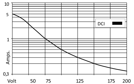
Fig. 3. DC LOAD LIMIT CURVE
