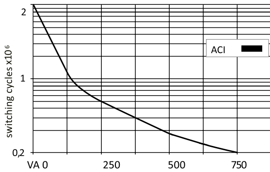
Fig. 2. AC VOLTAGE ENDURANCE
