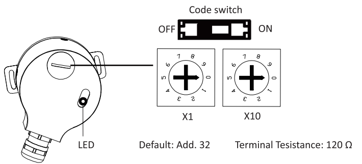
Encoder ID and terminal switch diagram
